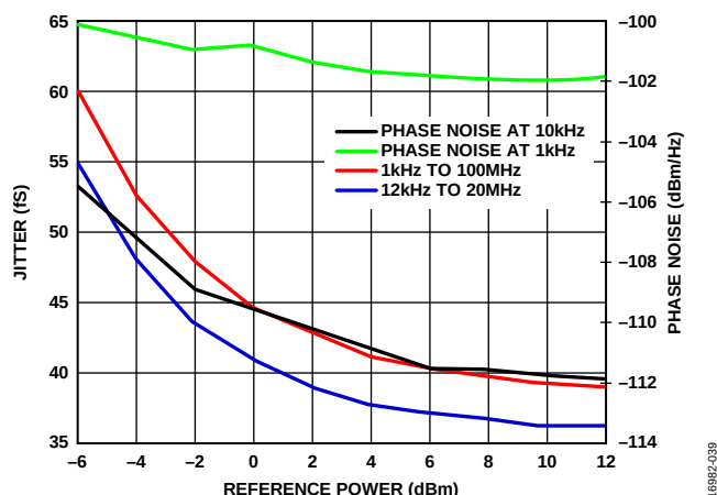
Figure 33. Jitter and Phase Noise, f_{PFD} = 250 MHz
