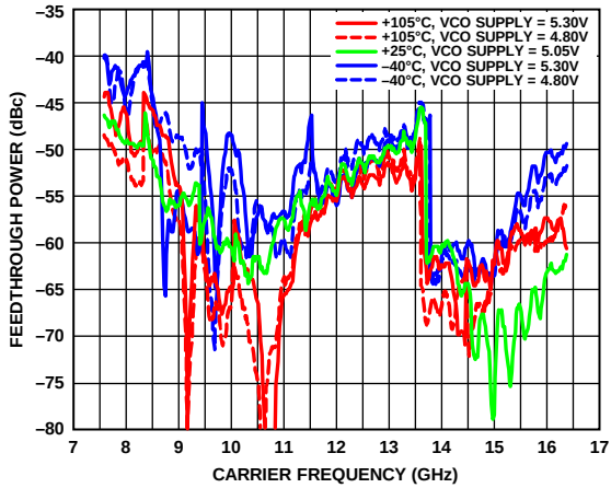
Figure 19. RF16P and RF16N VCO \times 3 Feedthrough, De-Embedded Board and Cable Measurement, Combined Using Balun
