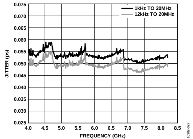
Figure 27. RMS Jitter, Fractional-N, f_{PFD} = 153.6 MHz, V_{CC\_VCO} = 5 V
