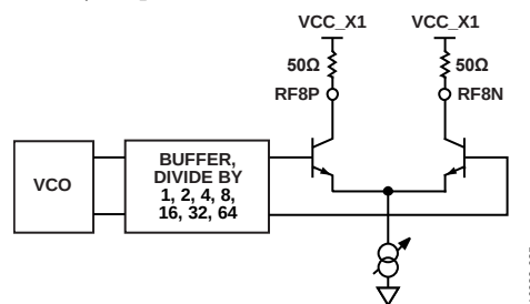
Figure 41. Output Stage
