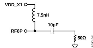
Figure 44. Optimum Output Stage
