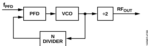
Figure 32. Loop Closed Before Output Divider
